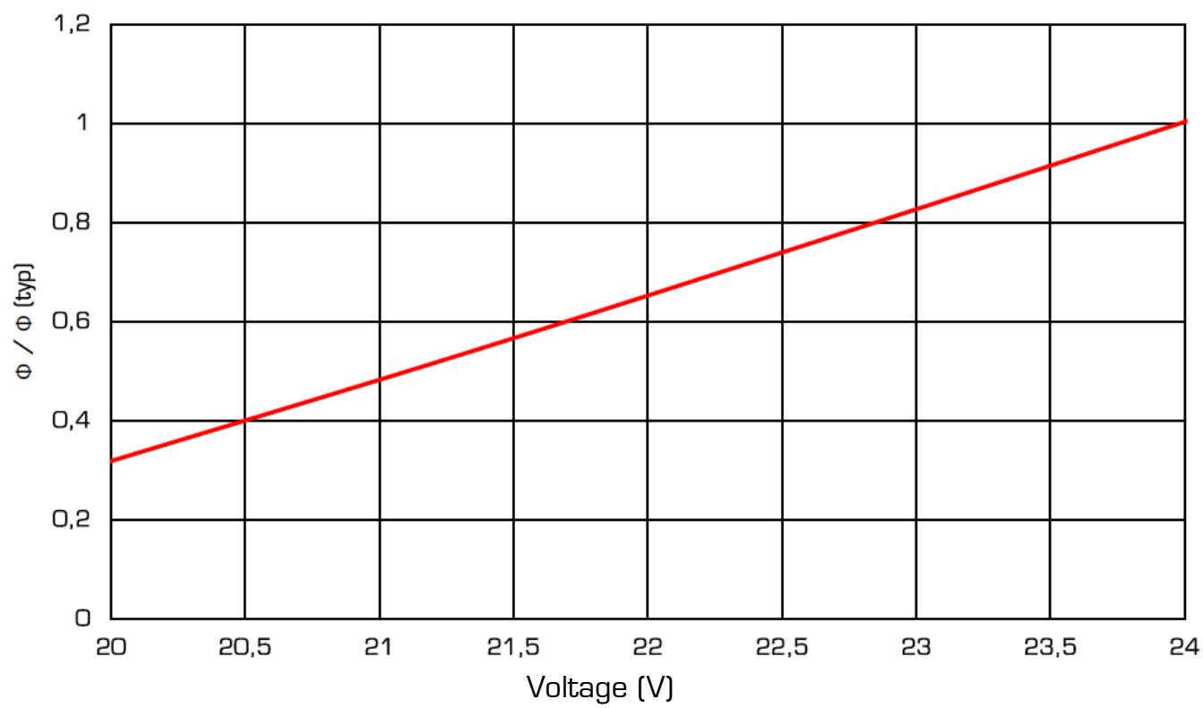
LUMINOUS FLUX vs. VOLTAGE
