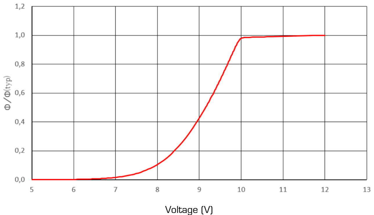
LUMINOUS FLUX vs. Voltage
