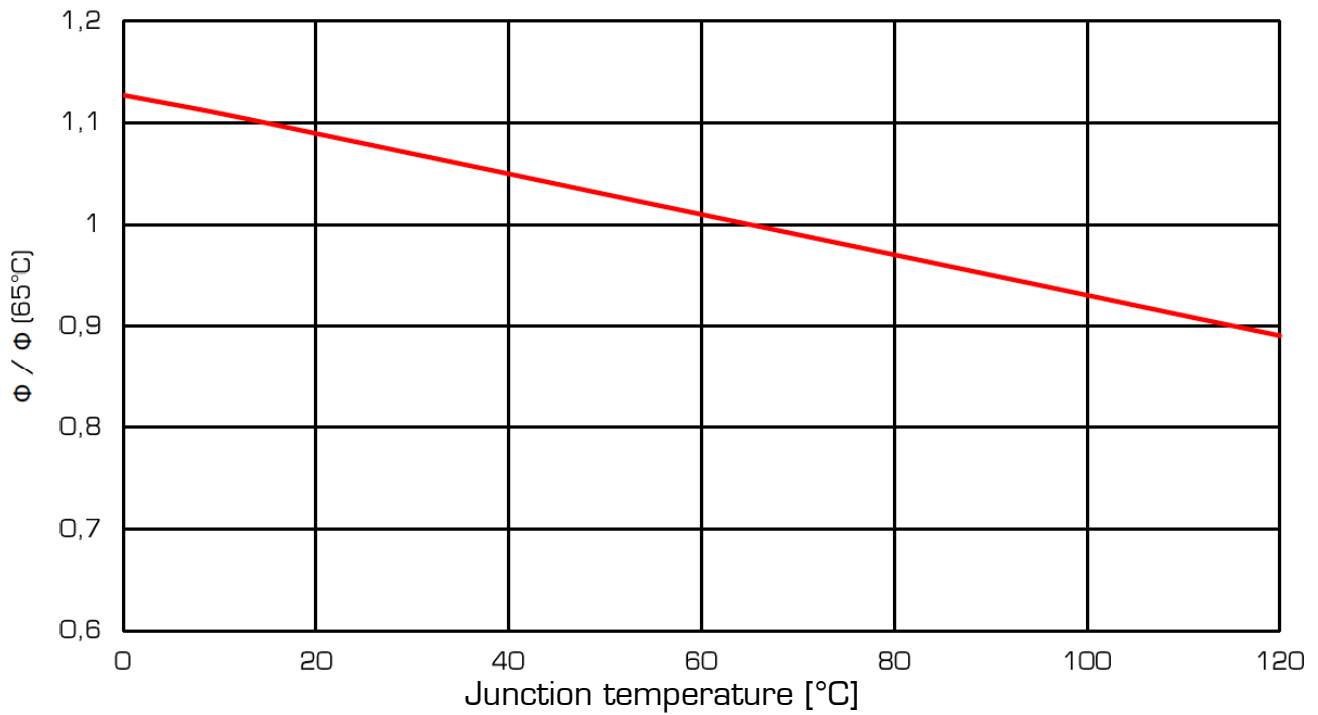
LUMINOUS FLUX vs. TEMPERATURE
