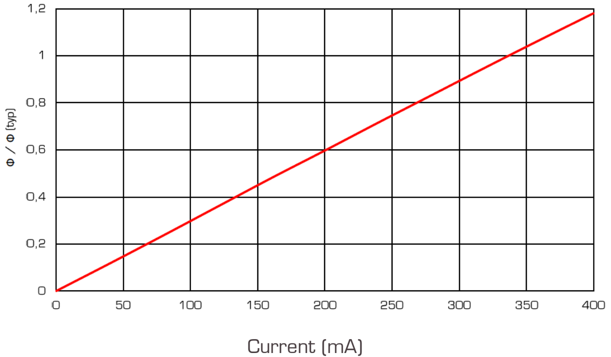
LUMINOUS FLUX vs. CURRENT
