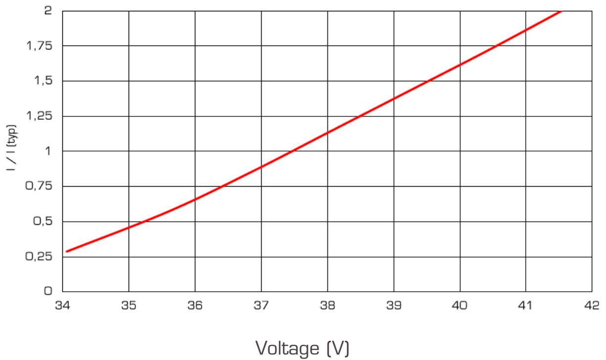
CURRENT vs. VOLTAGE
